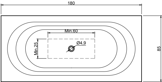
(Vasca centrale / Centered bathtub) art. OASI74MC peso lordo/gross weight: kg 149 ca peso netto/net weight: kg 124 ca
